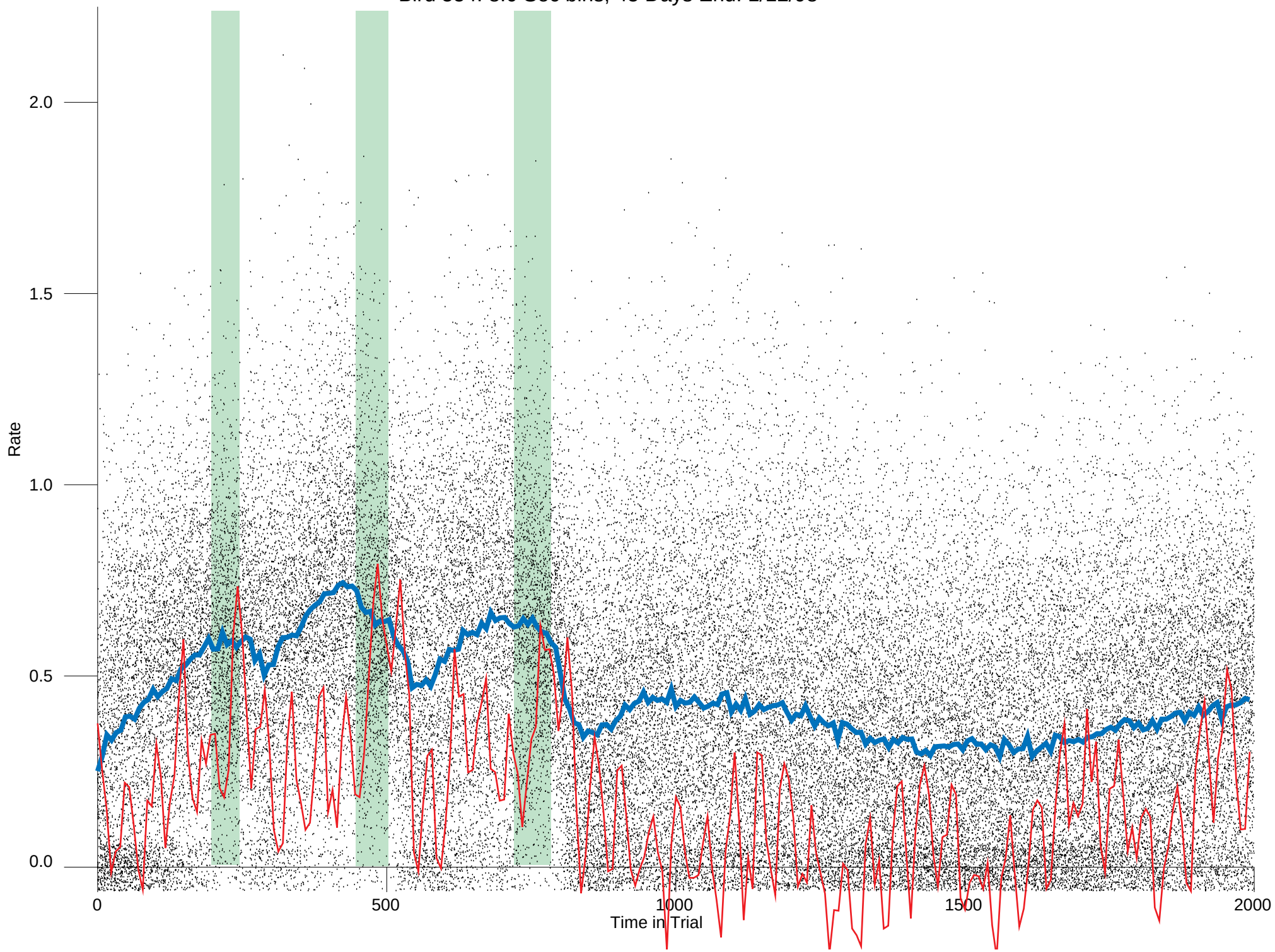
Bird 554: 8.0 Sec bins, 45 Days End: 1/12/98
