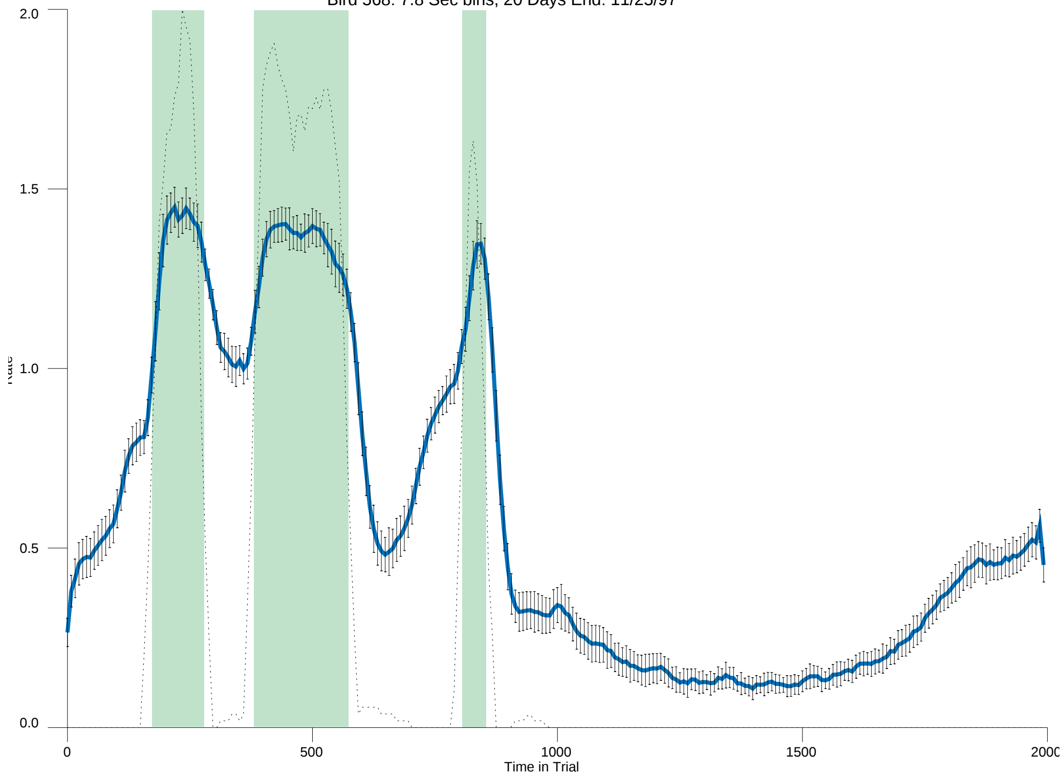
Bird 568: 7.8 Sec bins, 20 Days End: 11/25/97
