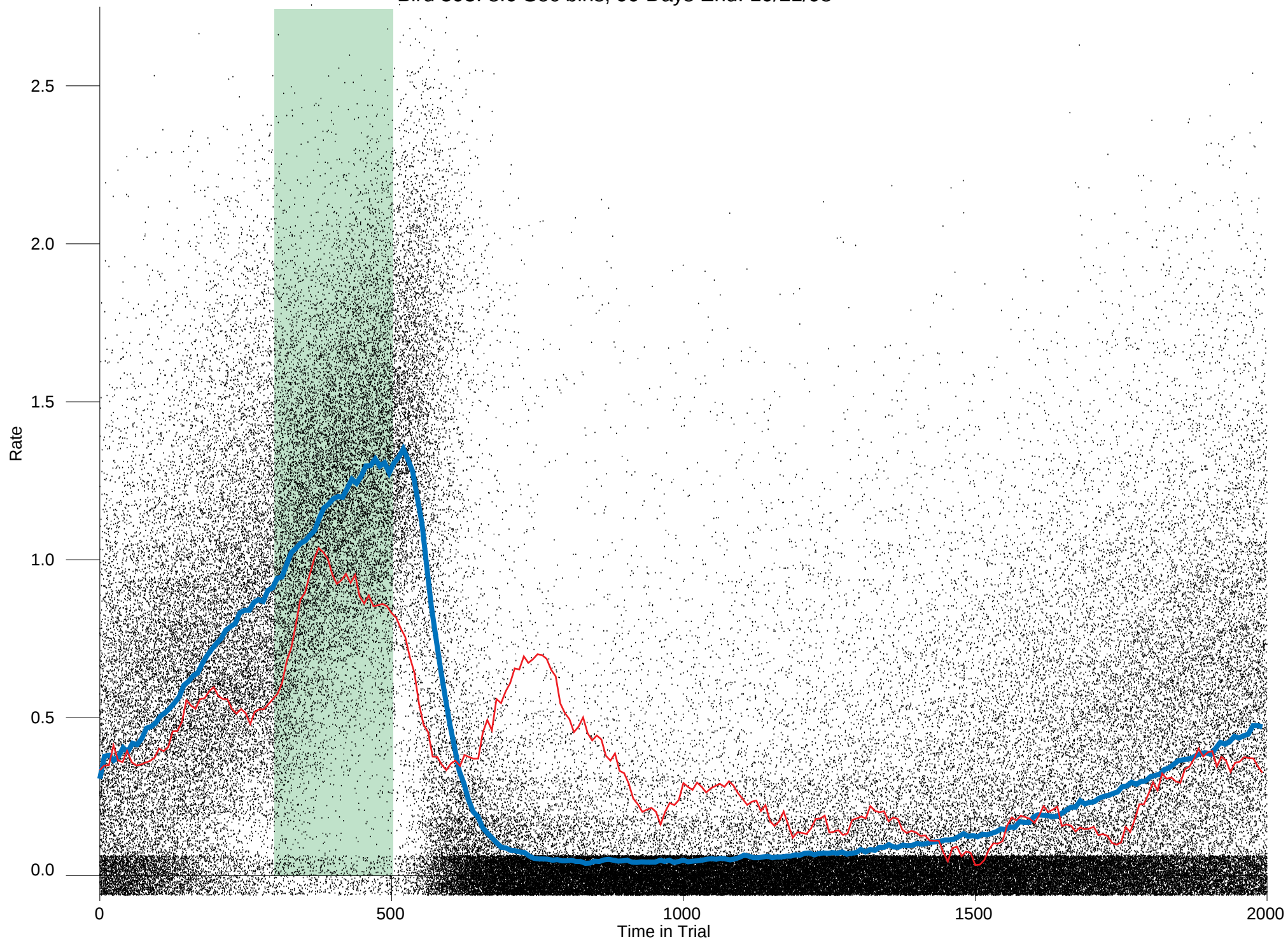
Bird 593: 8.0 Sec bins, 99 Days End: 10/21/98
